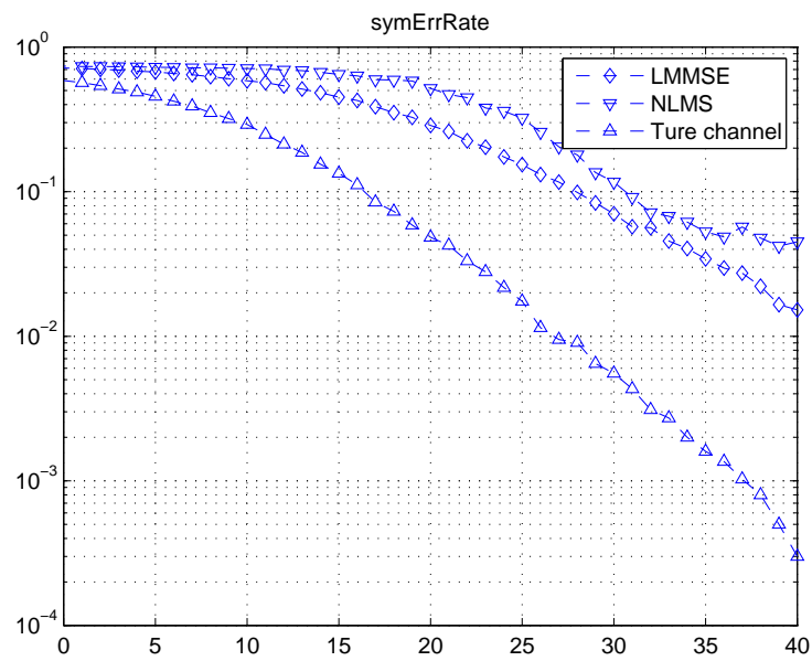
Figure 5.4: Simulation result under 50km/h (Part2)
