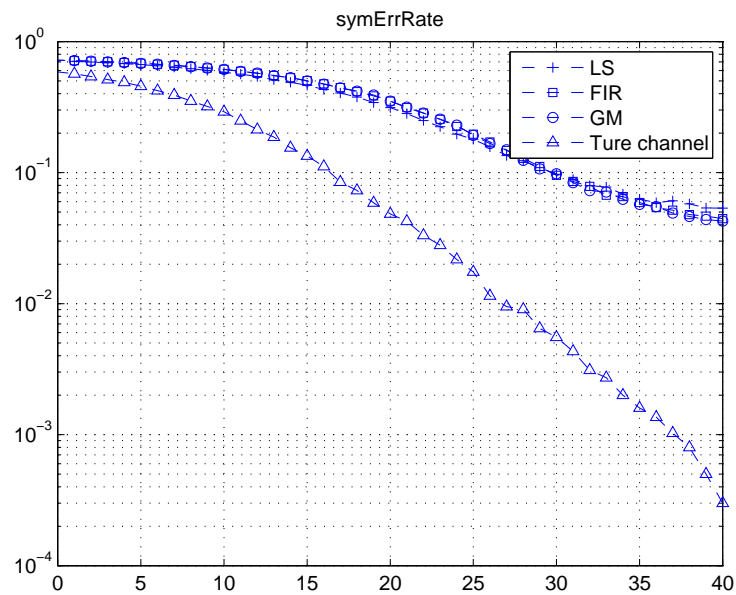
Figure 5.5: Simulation result under 120km/h (Part1)
