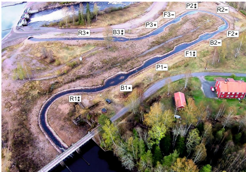
Figure 3. The biocanal before modifications of the channel. Abbreviations; R = riffle, B = braided, P = pool, F = floodplain. - indicates habitats in which no LWD was added, one star indicates habitats in which a low density of LWD later was added and two stars indicates habitats in which a high density of LWD later was added. Photo: Anders Bruks
